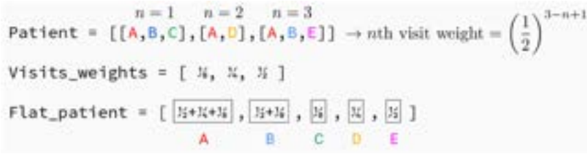
Fig. 4. Example of temporal encoding for a patient.
