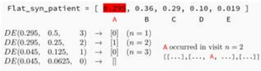
Fig. 5. Example of temporal decoding for a patient.
